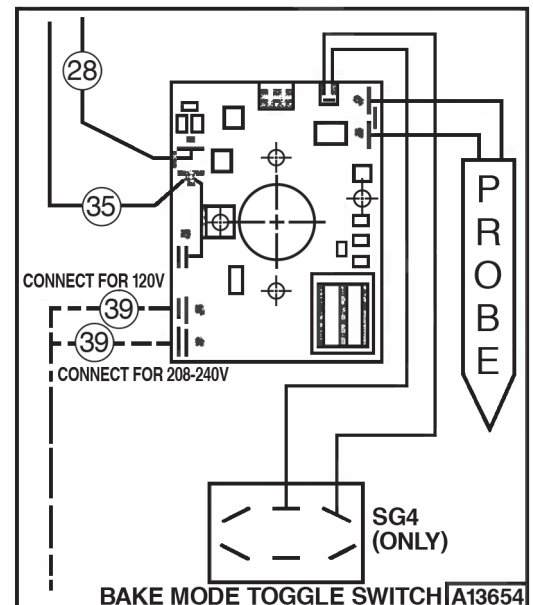
Wiring Diagram
