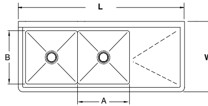
2 COMP - 1 DRBD
