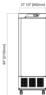
QVR(F)-1 Front View
