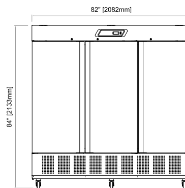
QVR(F)-3 Front View
