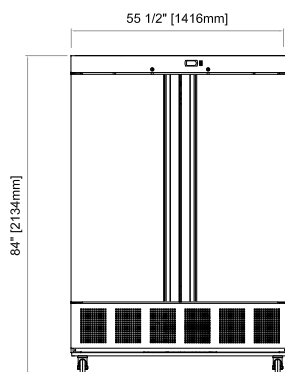
QVR(F)-2 Front View
