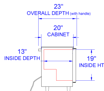
END VIEW UCR/UCF20 END
