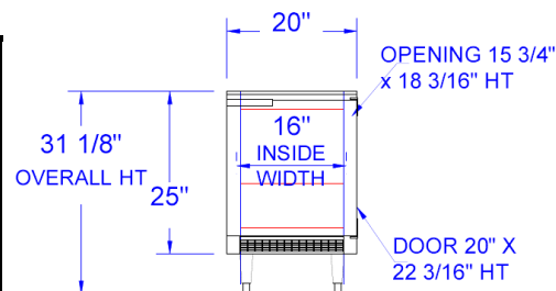
FRONT VIEW UCR/UCF20 FRONT
