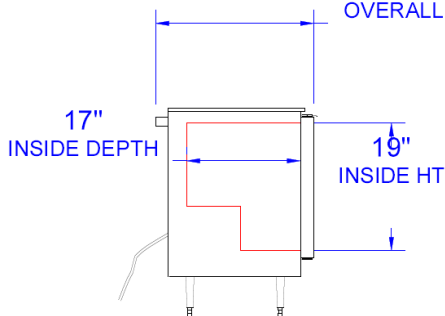
LEFT SIDE VIEW UCR34 FRONT
