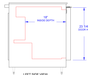
LEFT SIDE VIEW UCR/UCF27 END
