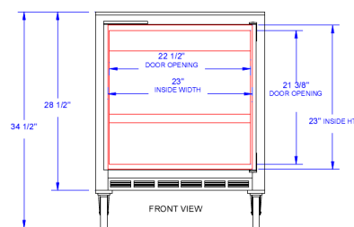
FRONT VIEW UCR/UCF27 FRONT
