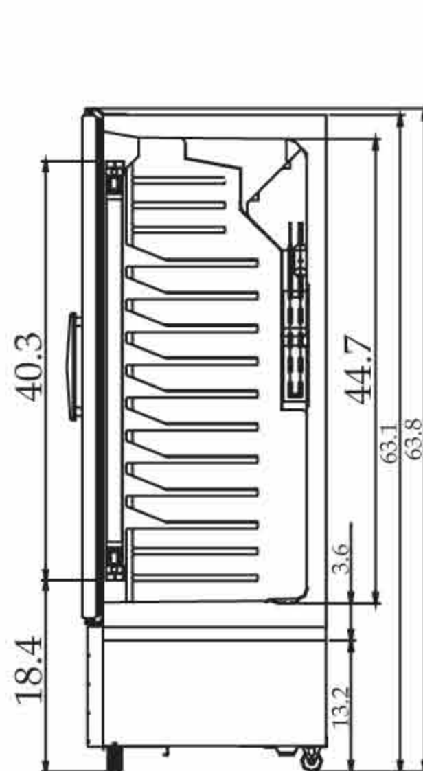
TGM-11RV SIDE VIEW
